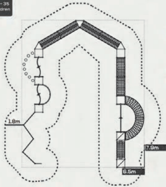
Top View - Safe Use Zone
