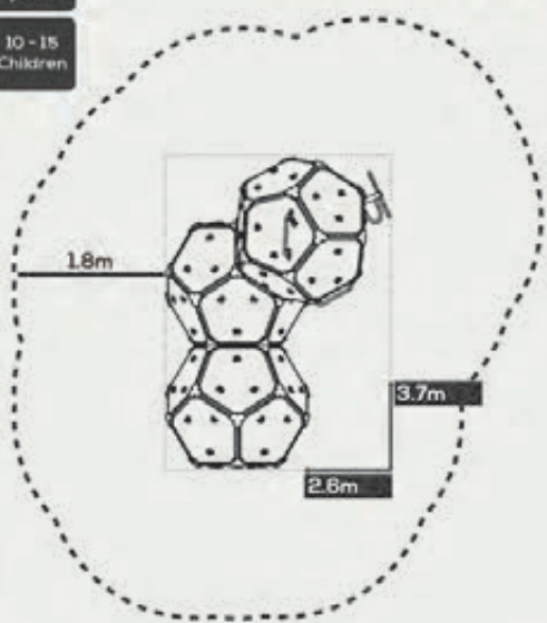
Top View - Safe Use Zone
